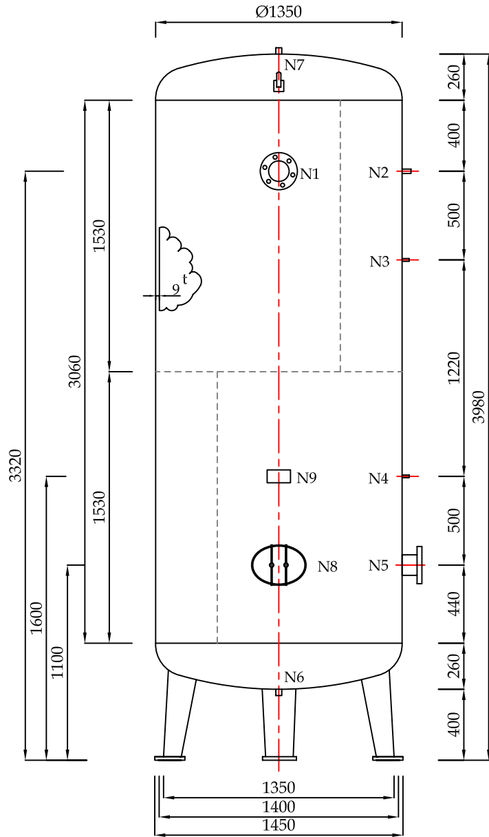
FRONT VIEW
